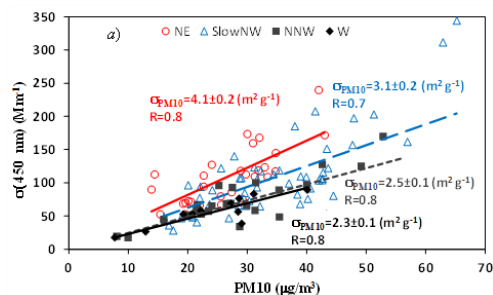
Figure 1. Scattering coefficient versus PM10 mass concentrations.
