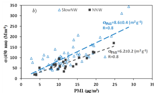
Figure 2. Scattering coefficient versus PM1 mass concentrations.
